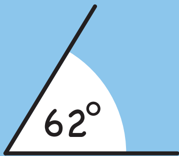
spitzer Winkel
